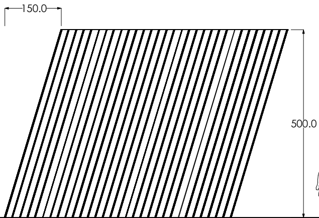
Elevation 1/200 dimensions in cm
